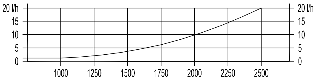
Consumo de combustible Fuel Flow
